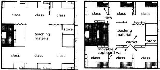
1 Schoolroom without walls
